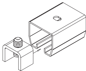
Adjustable Track End Stop
