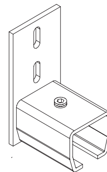
Wall Mount End Stop - Flange Up
