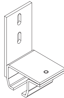
Split Support Bracket Flange Up
